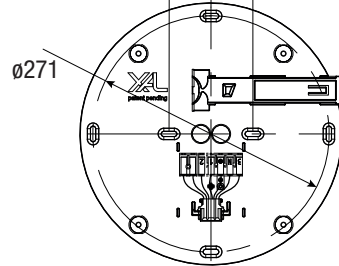
MOUNTING DIMENSIONS VELA EVO 450 / 600 6 x SCREW
