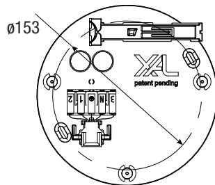
MOUNTING DIMENSIONS VELA EVO 300 2 x SCREW
