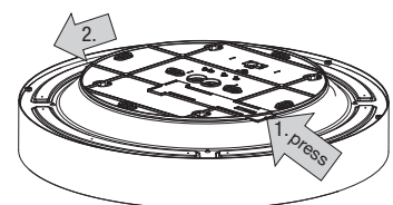
Dismounting Vela Evo Surface | Ceiling 300 / 450 / 600 / 900 / 1200
