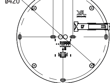
MOUNTING DIMENSIONS VELA EVO 900 / 1200 6 x SCREW
